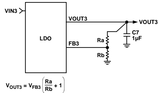
Figure 48. LDO External Output Voltage Setting
